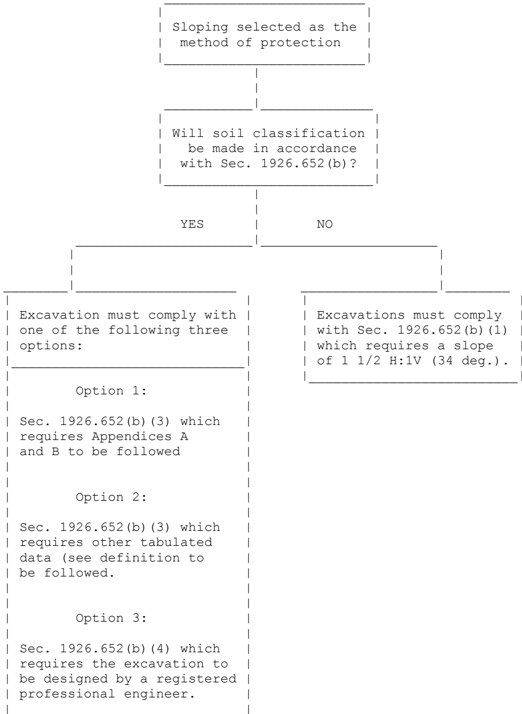
Figure 3. Shoring and Shielding Options
