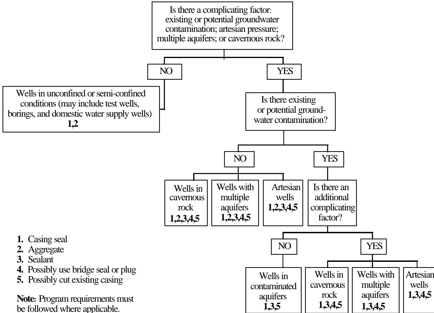
Figure 10. Summary of procedures for well abandonment.
